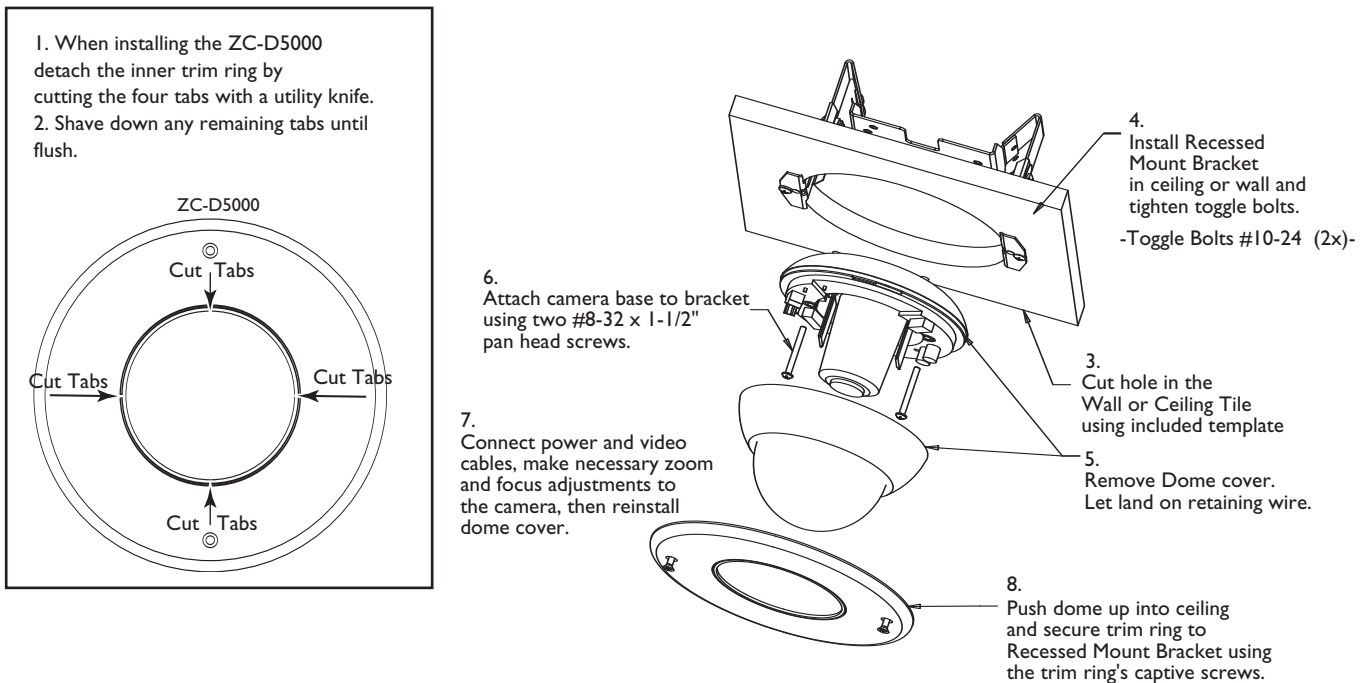
Fig. 3 Installing Recessed Mount Kit ZC-D5000 Series Dome
