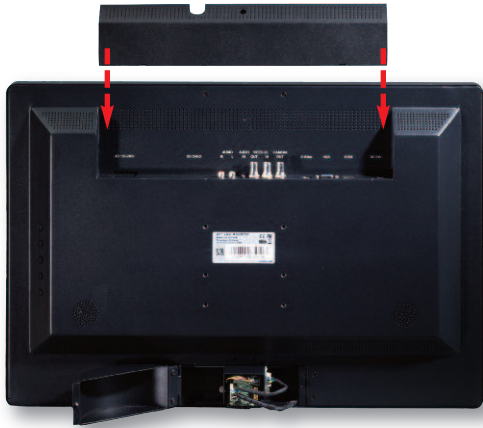
Input Panel (Cover Removed)
